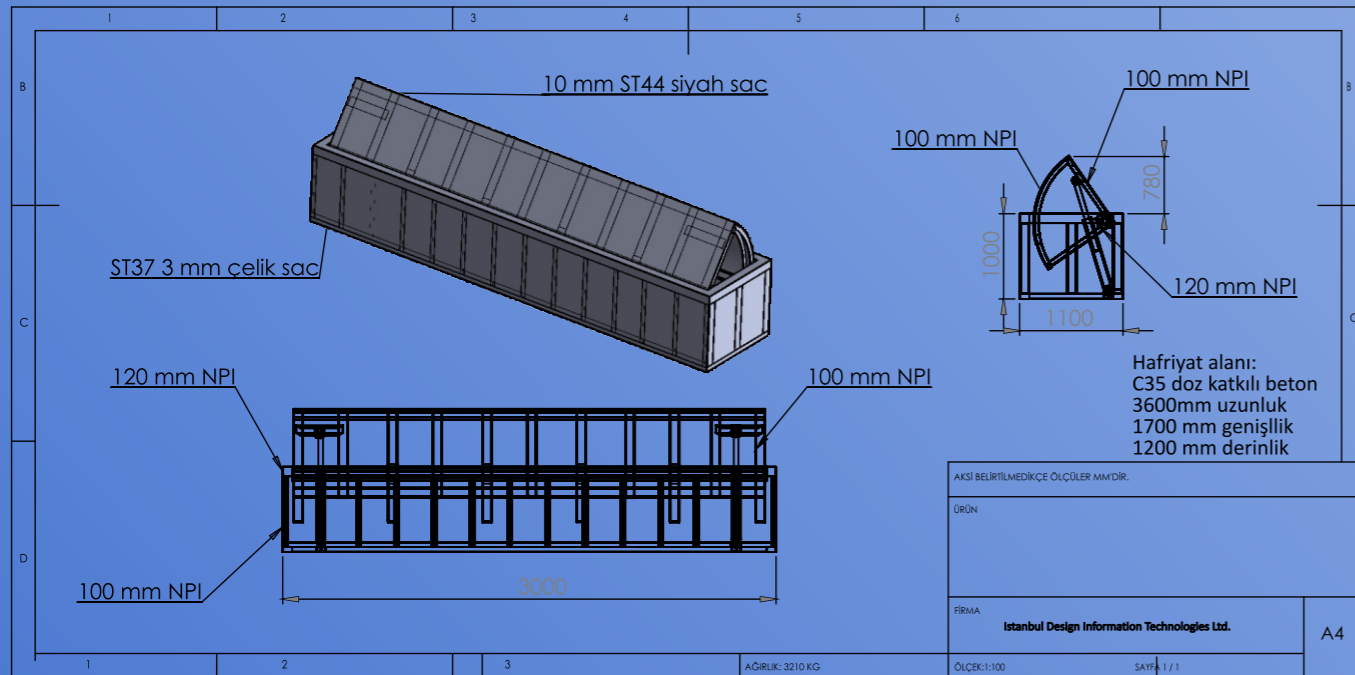
Technical Dimensions
